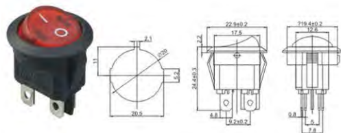
A-TOP1-8-201 ON-OFF A-TOP1-8-201N-X ON-OFF With Light
